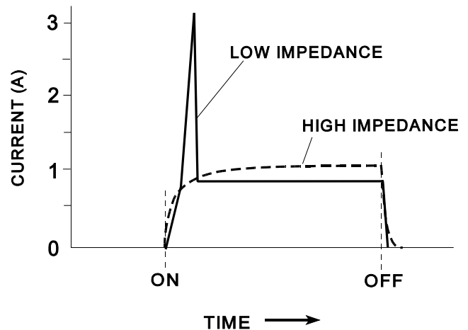
Typical Injector Drive Current Waveforms
